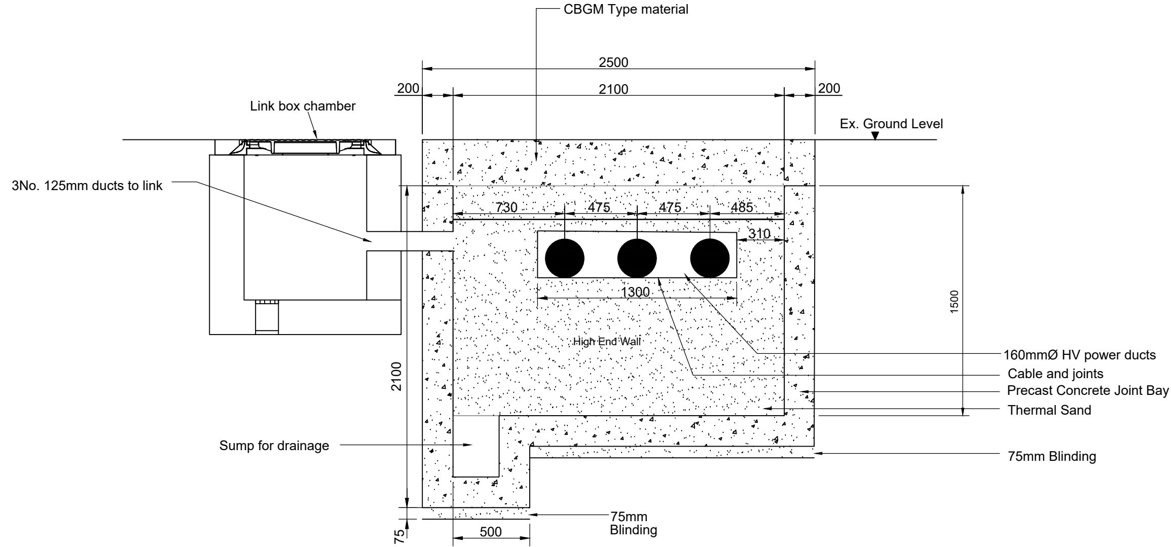
Section B-B
