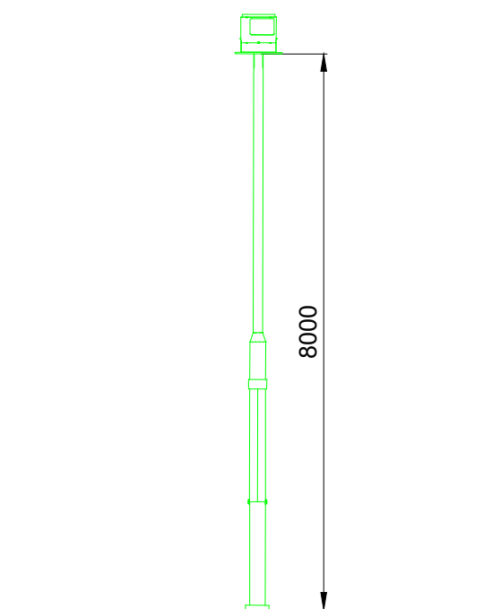
PROPOSED SECTION OF NEW LIGHTING MONOPOLE SCALE : 1:100
