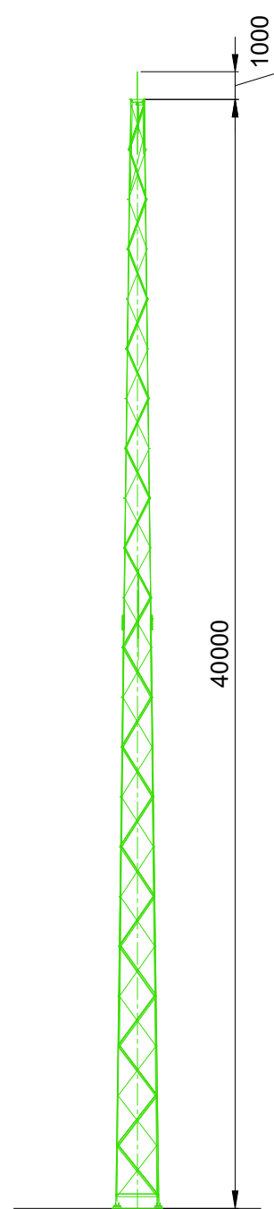
PROPOSED SECTION OF NEW LIGHTNING MAST SCALE : 1:250
