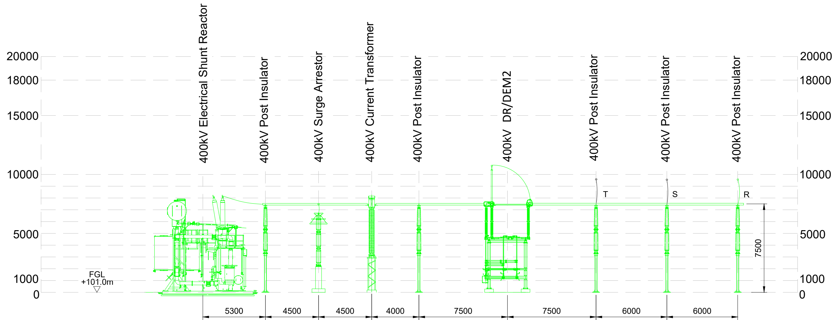
SECTION B-B SCALE 1:200
